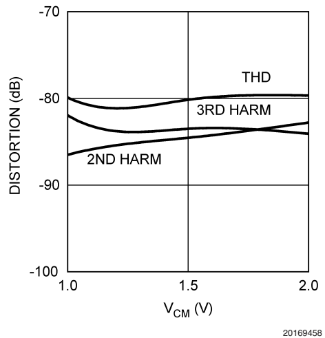
Distortion vs. V_{CM}
