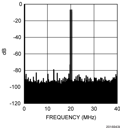
Intermodulation Distortion, f_{IN1} = 19.6 MHz, f_{IN2} = 20.2 MHz
